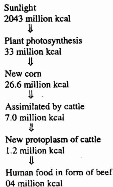
Figure 1: Energy flow in a cornfield in a field lot (Based on Transeau 1926 and Heichel 1976)
